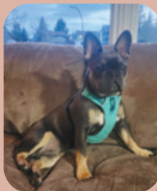
Coco, Shawnessy
